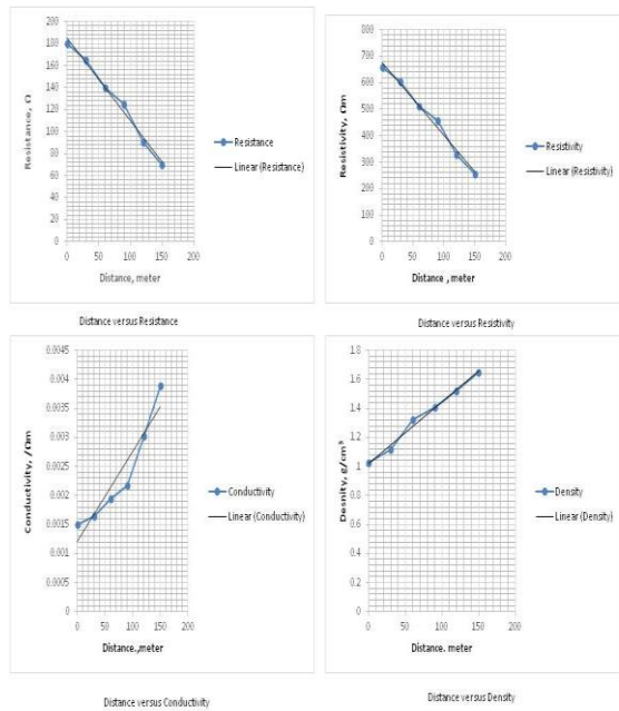
Fig.5. Resistance, Resistivity, Conductivity and Density
